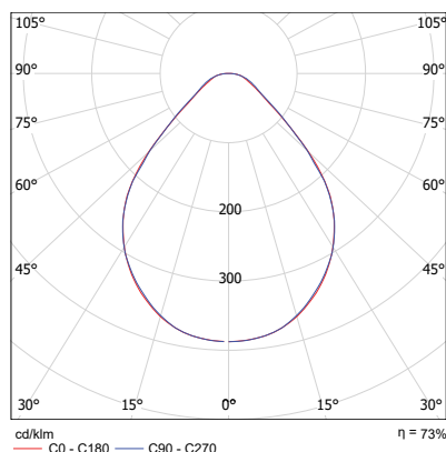
Ledge recessed micro 600x600 42W
