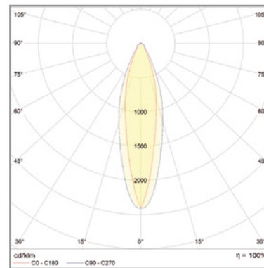
Narrow beam 30°
