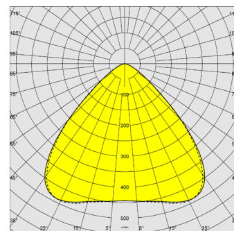
Diffuser for UGR<22 opal or transparent.
