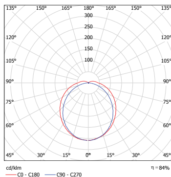
Proof opal kuppel
