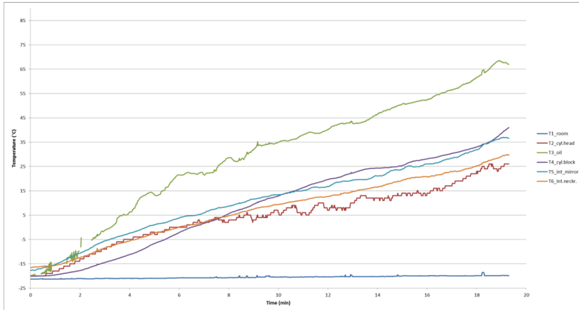
Figure 2. Measured temperatures during the test cycle F1.
