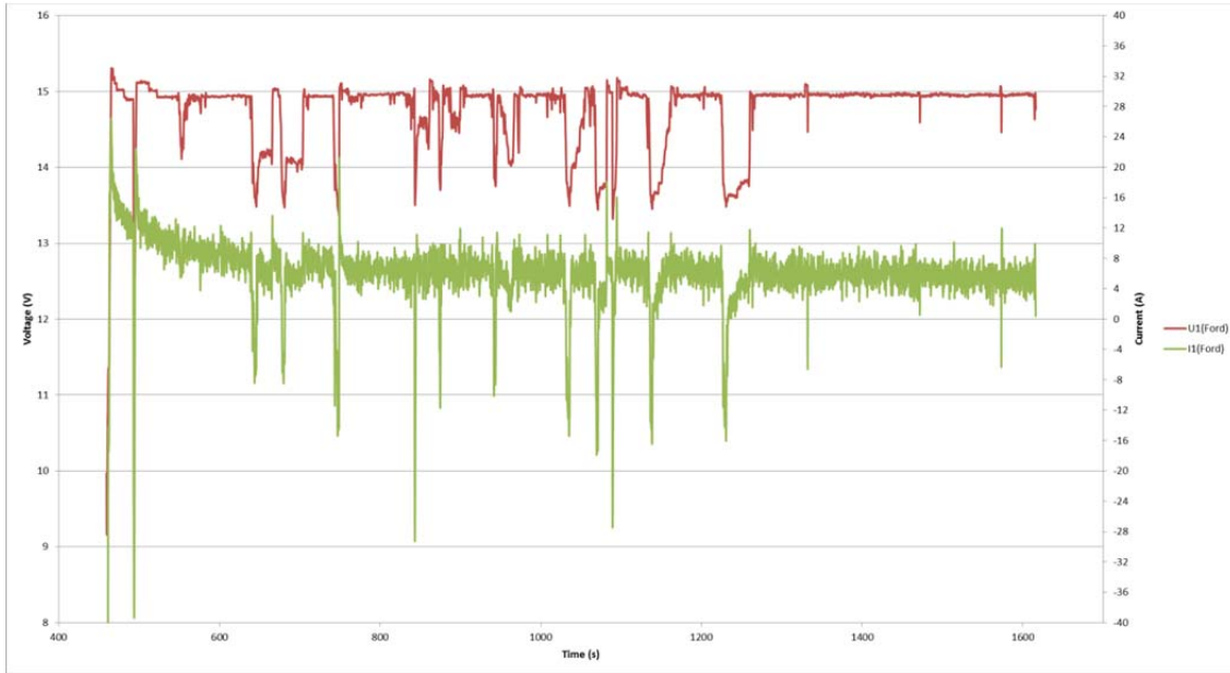
Figure 3. The voltage/current graph of test F1.
