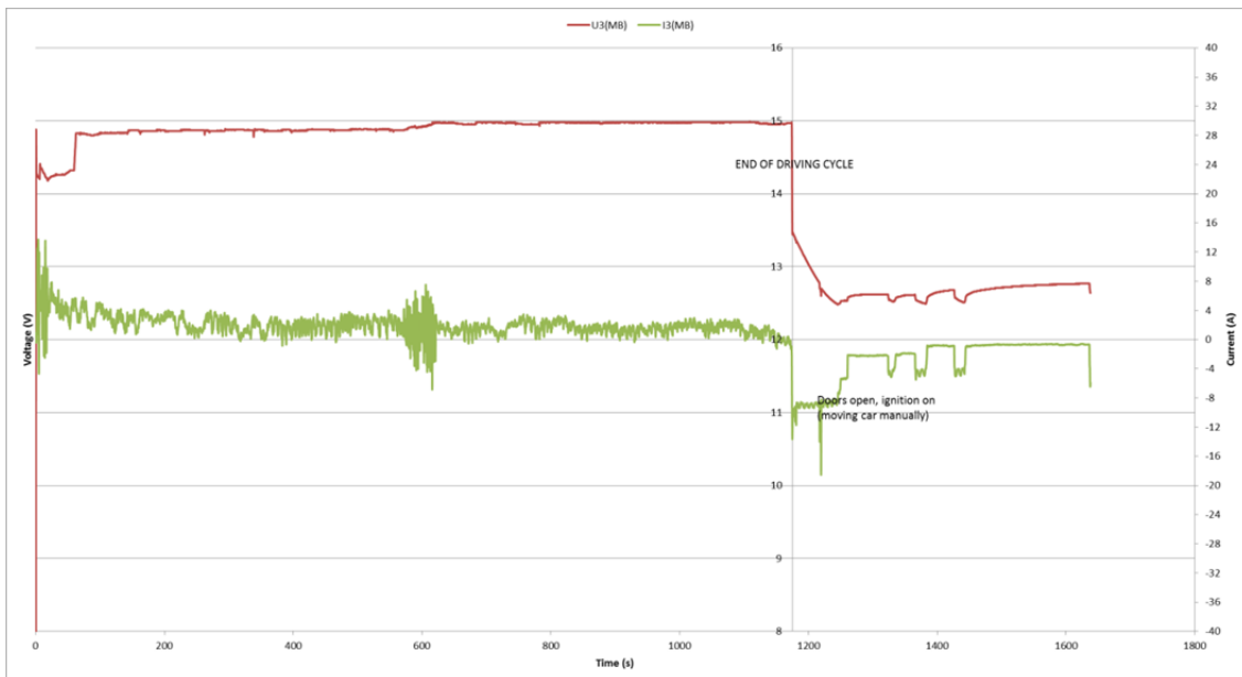
Figure 5. The voltage/current graph of test 5 during the driving cycle.
