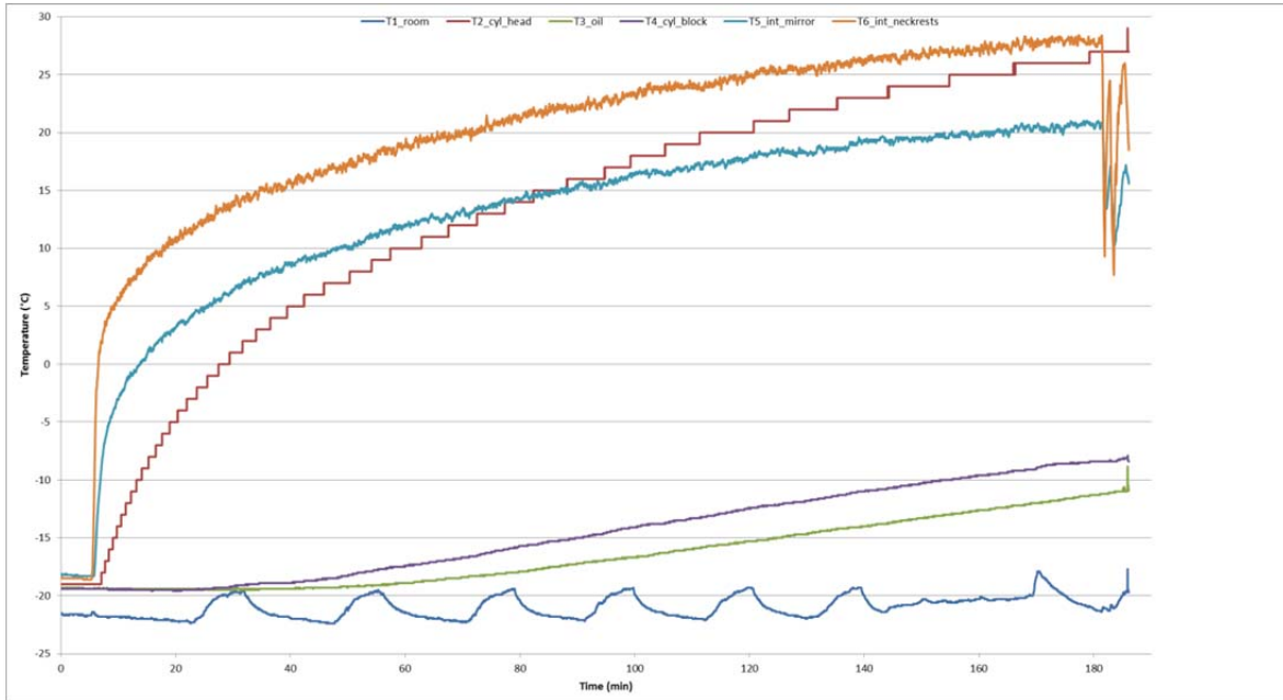
Figure 2. Measured temperatures during the preheating period of test D5.
