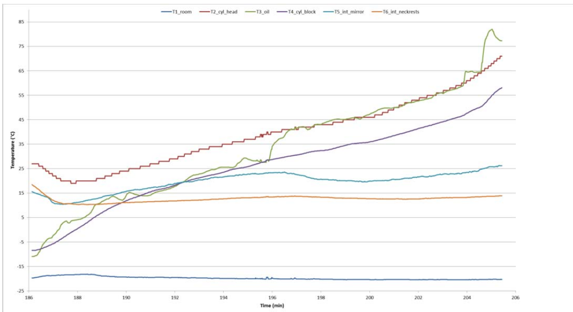
Figure 3. Measured temperatures during the driving cycle of test D5.
