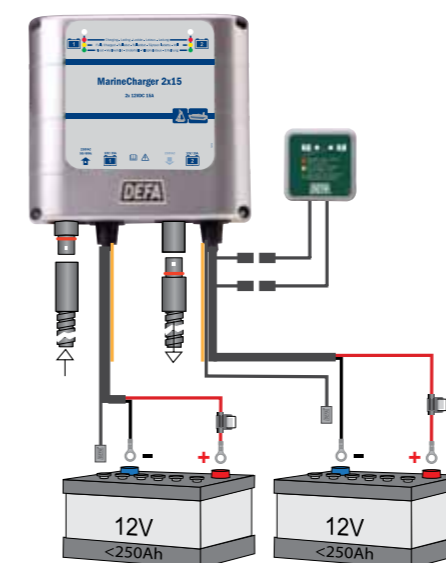
24V System
