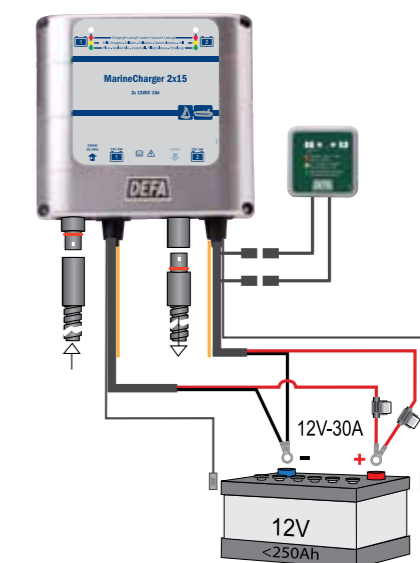
12V System
